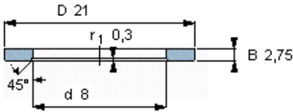
Universal washer
